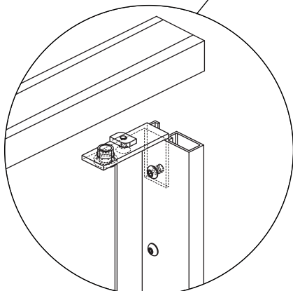
Overhead-Bracing Headrail
